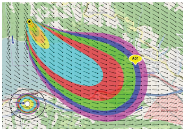
Exercise Control (EXCON) showing plume release, radiological “hot spot”, simulated wind field and student surveyor (icon A01).
